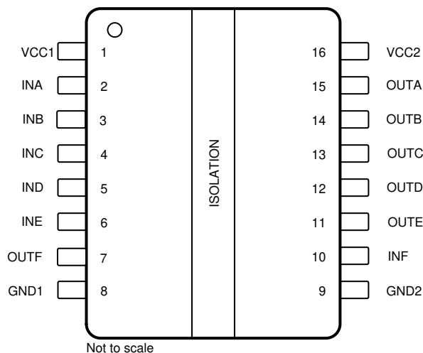
图 5-2. ISO6761 DW Package 16-Pin SOIC-WB Top View
