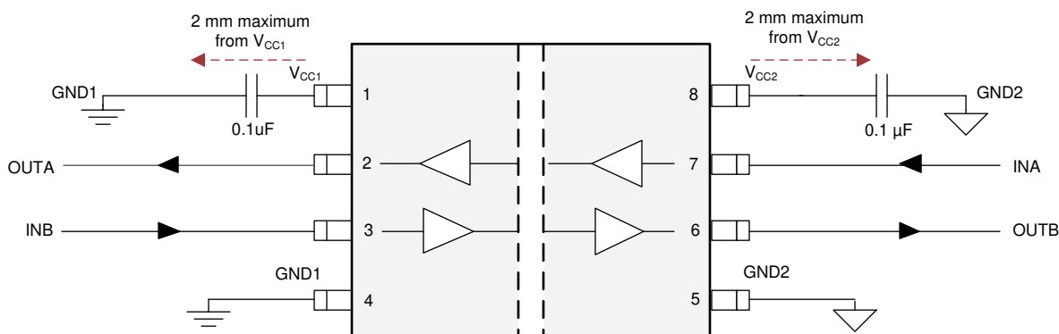
图 9-2. Typical ISO672xB Circuit Hook-up
