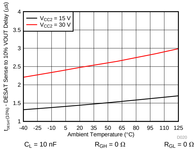
Figure 33. DESAT Sense to V_{\text{OUT}} 10% Delay vs Temperature
