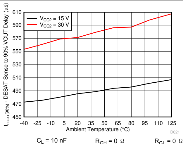
图 7-34. DESAT Sense to V_{OUT/IL} 90% Delay vs Temperature
