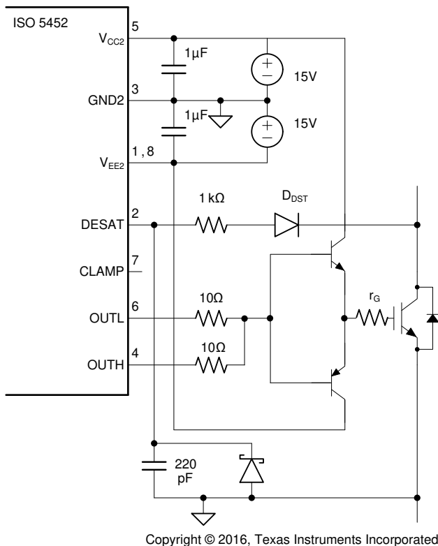
图 10-10. Current Buffer for Increased Drive Current
