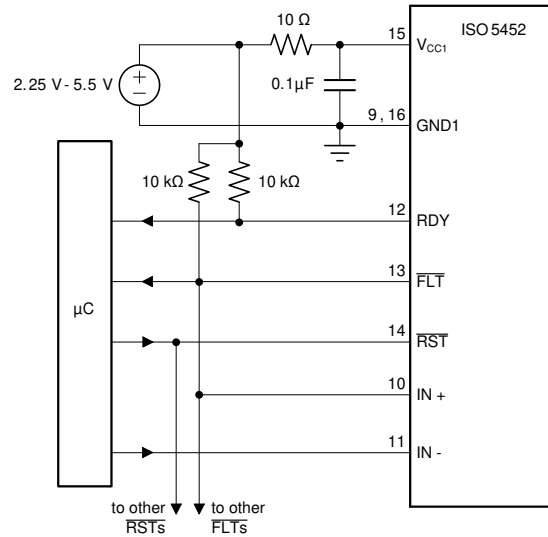
图 10-6. Global Shutdown With Inverting Input Configuration
