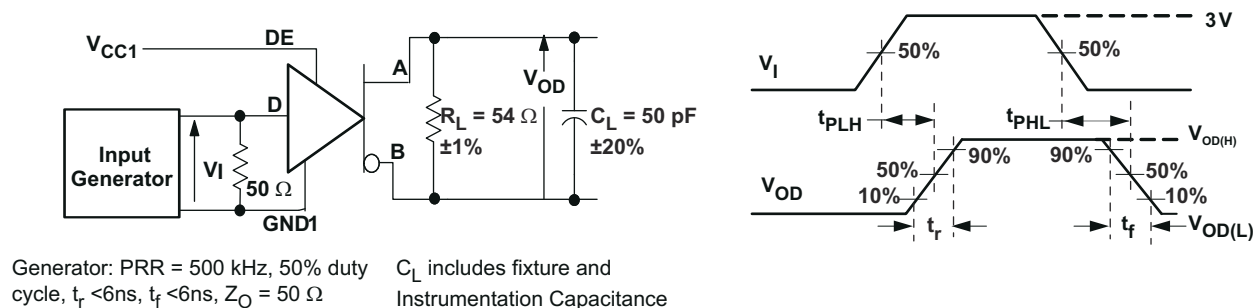
图 7-4. Driver Switching Test Circuit and Voltage Waveforms
