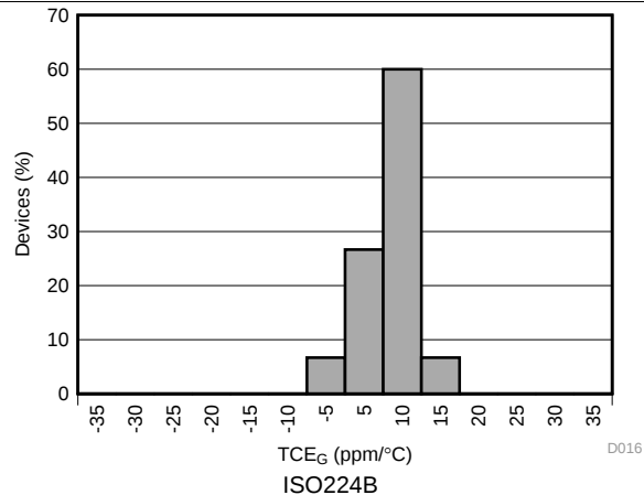
图 18. Gain Error Drift Histogram
