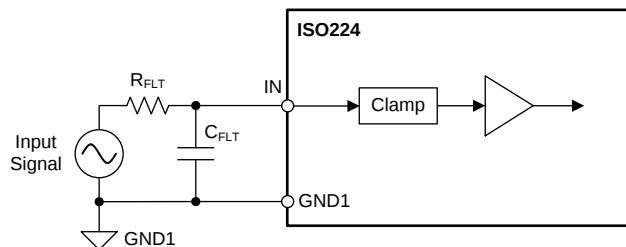
图 43. Series Resistor-Based Input Current Limitation on the Analog Inputs of ISO224
