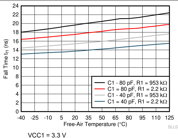
Figure 6-9. Side 1: Output Fall Time vs Free-Air Temperature
