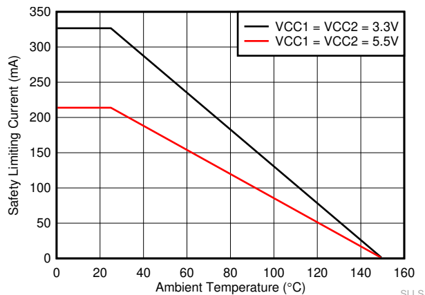
图 6-1. Thermal Derating Curve for Safety Limiting Current for D-8 Package
