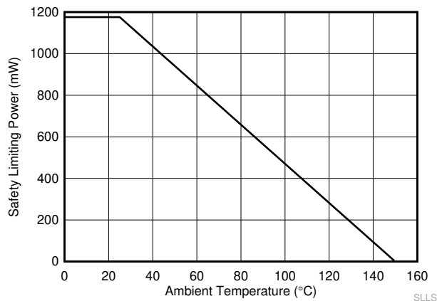
图 6-2. Thermal Derating Curve for Safety Limiting Power for D-8 Package
