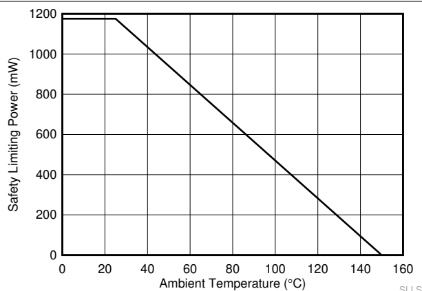
图 6-4. Thermal Derating Curve for Safety Limiting Power for DW-16 Package
