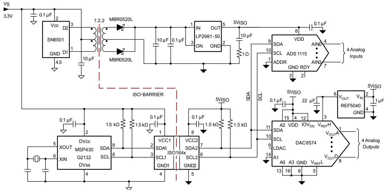
图 9-4. Isolated I 2 C Data Acquisition System
