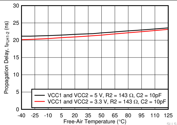
图 6-13. t_{PLH1-2} Propagation Delay vs Free-Air Temperature
