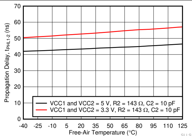
图 6-15. t_{PHL1-2} Propagation Delay vs Free-Air Temperature
