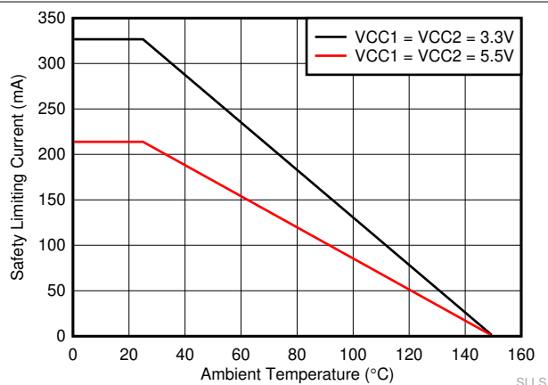
图 6-3. Thermal Derating Curve for Safety Limiting Current for DW-16 Package
