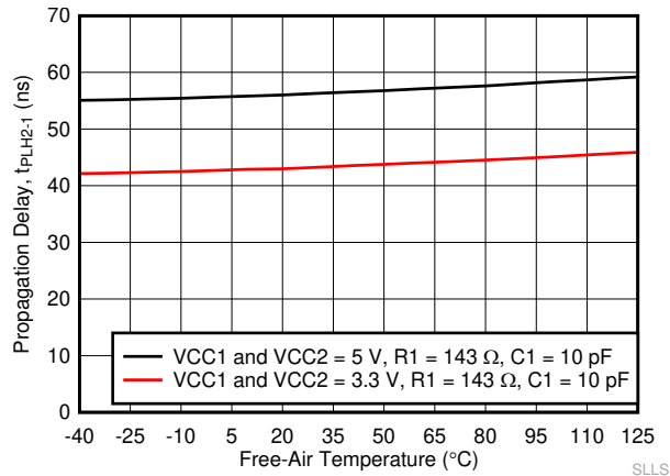
图 6-17. t_{PLH2-1} Propagation Delay vs Free-Air Temperature
