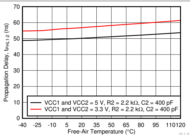
Figure 6-16. t_{PHL1-2} Propagation Delay vs Free-Air Temperature
