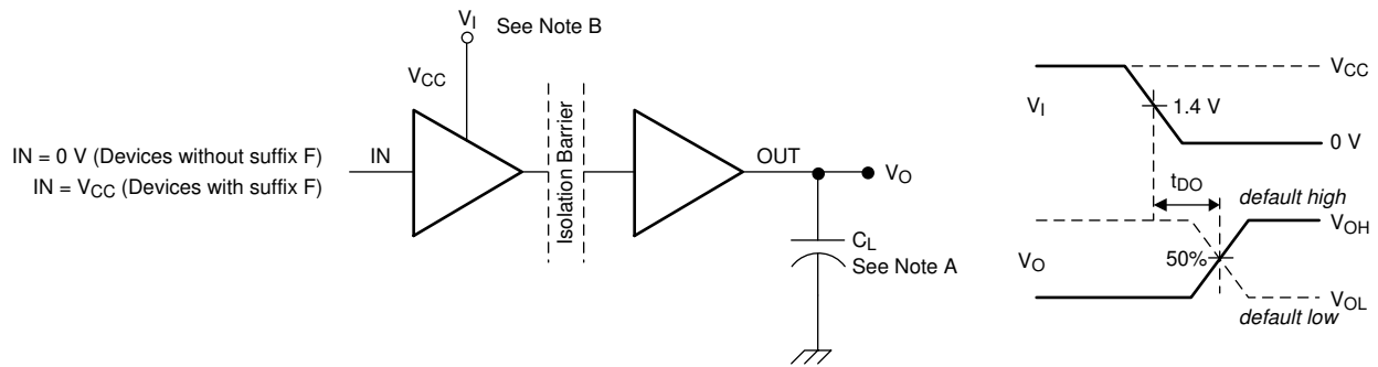
Figure 7-4. GPIO Channel Switching Characteristics Test Circuit and Voltage Waveforms
