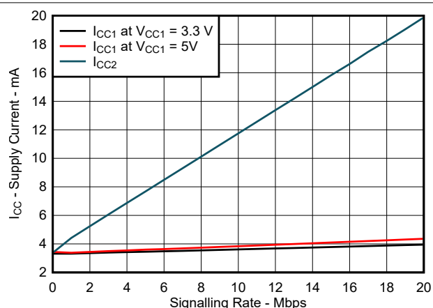
图 6-3. RMS Supply Current vs Signaling Rate
