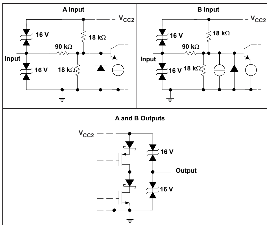
图 8-2. Equivalent I/O Schematics for A and B Inputs and Outputs
