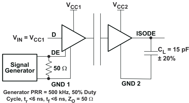
图 7-14. DE to ISODE Prop Delay Test Circuit and Waveforms
