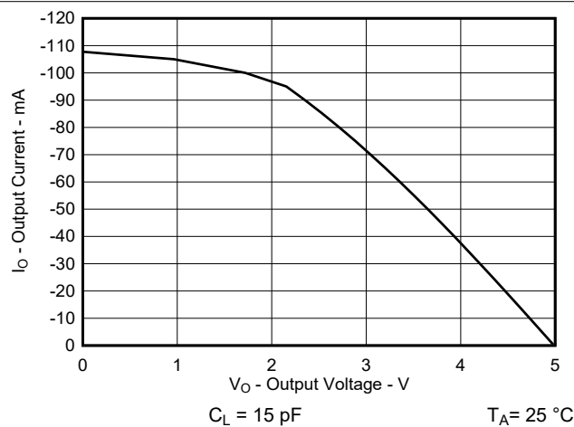
图 6-7. High-Level Output Voltage vs High-Level Output Current
