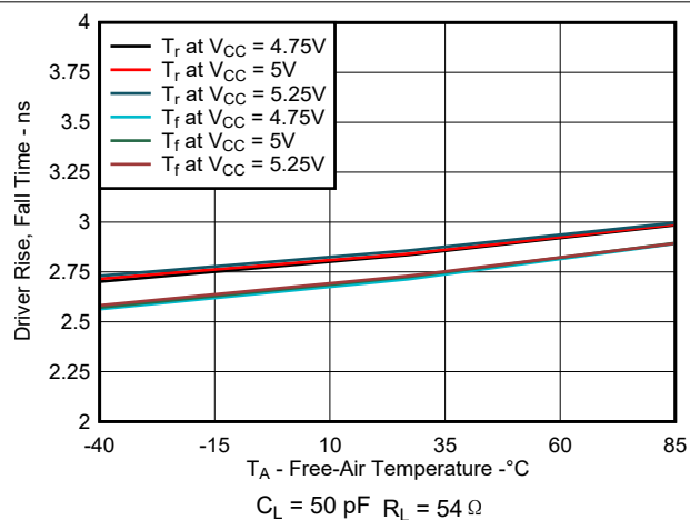
图 6-5. Driver Rise and Fall Time vs Free-Air Temperature
