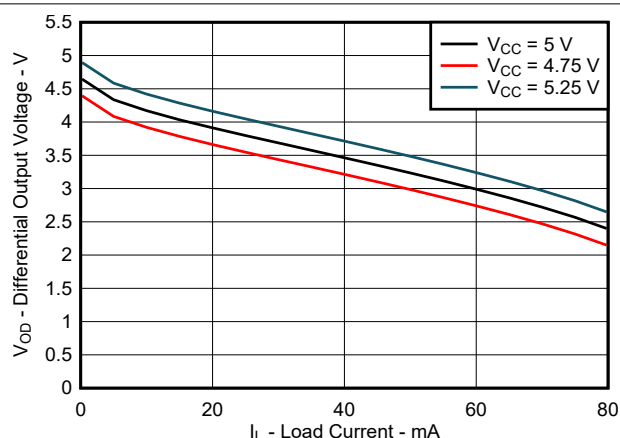
图 6-2. Differential Output Voltage vs Load Current
