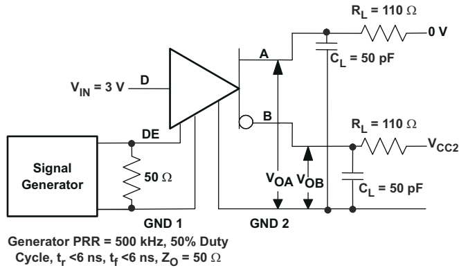
图 7-13. Driver Enable and Disable Test, D at Logic High Test Circuit and Waveforms
