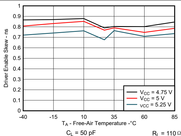
图 6-6. Driver Enable Skew vs Free-Air Temperature
