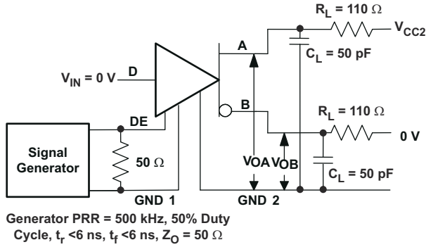
图 7-12. Driver Enable and Disable Test, D at Logic Low Test Circuit and Waveforms
