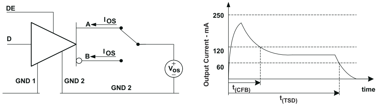
图 7-9. I_{OS(ss)} Steady State Short-Circuit Output Current Test Circuit
