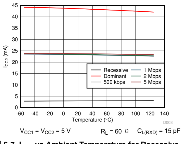
图 6-7. I_{CC2} vs Ambient Temperature for Recessive, Dominant and Different CAN Datarates
