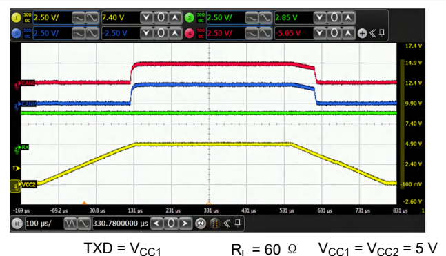
图 6-14. Glitch Free Power Up on V_{\text{CC2}} - CAN Bus Remains Recessive
