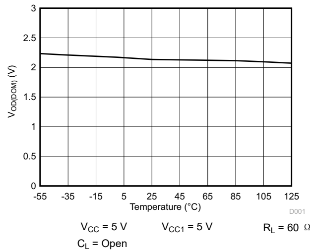
图 6-10. V_{\text{OD(DOM)}} Over Temperature
