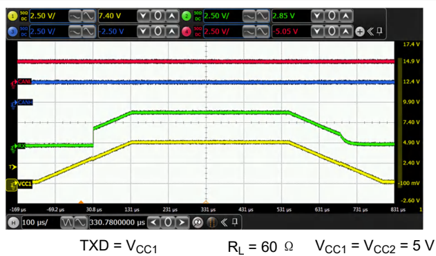
图 6-13. Glitch Free Power Up on V_{\text{CC1}} - CAN Bus Remains Recessive
