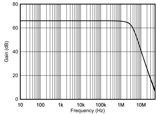
图 7-22. Closed Loop Gain vs Frequency
