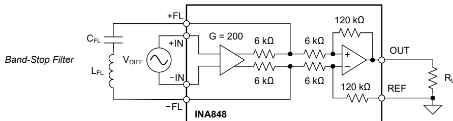
图 9-2. Bandstop Filter
