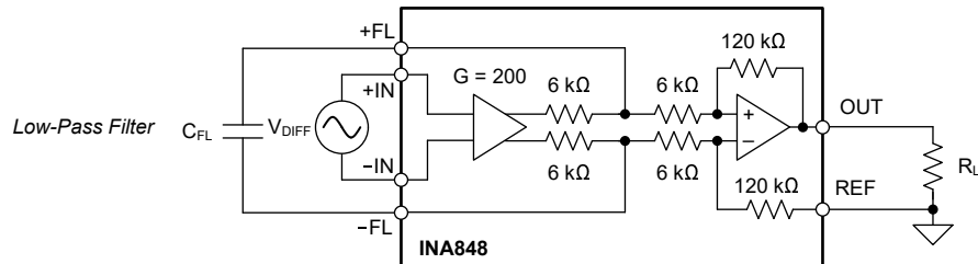
图 9-1. Low-pass Filter
