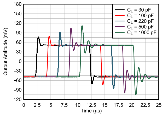
图 7-31. Small-Signal Response
