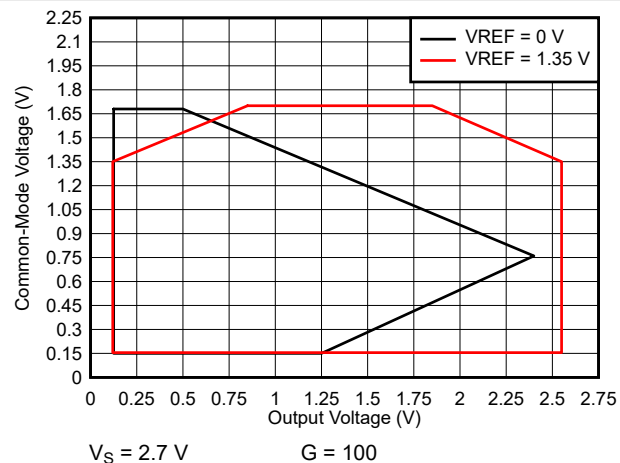
图 7-54. Input Common-Mode Voltage vs Output Voltage
