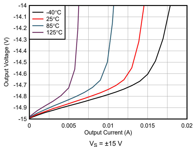
图 7-50. Negative Output Voltage Swing vs Output Current
