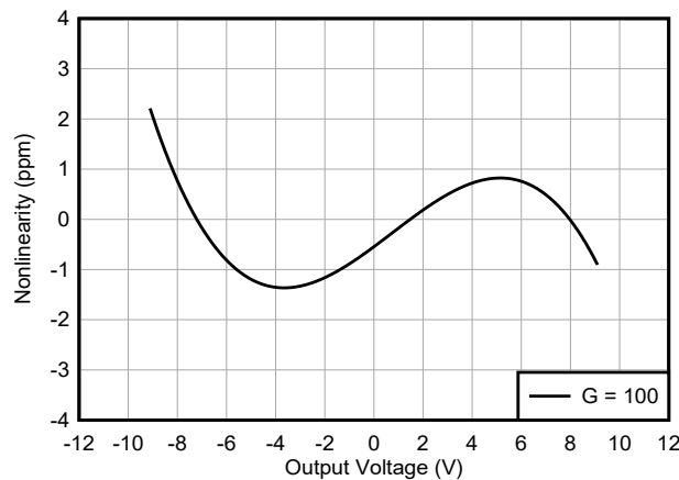
图 7-39. Gain Nonlinearity
