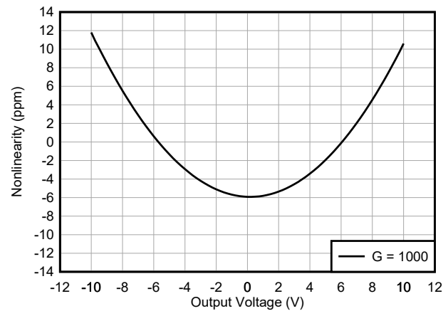
图 7-40. Gain Nonlinearity
