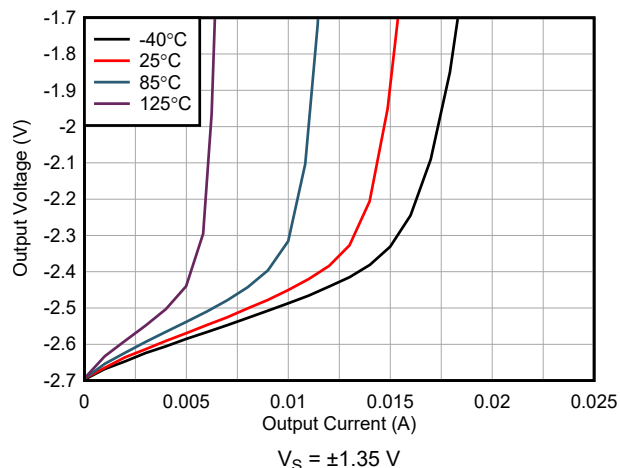
图 7-52. Negative Output Voltage Swing vs Output Current
