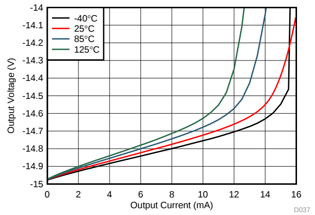
图 38. Negative Output Voltage Swing vs Output Current
