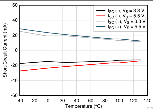
图 6-20. Short Circuit Current vs Temperature
