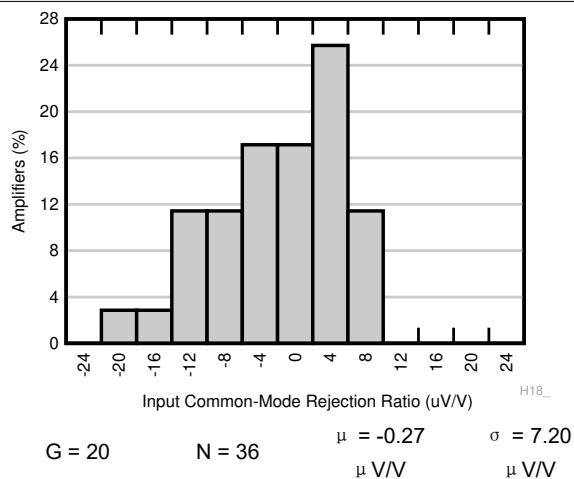
图 6-8. Typical Distribution of CMRR
