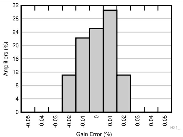
图 6-11. Typical Distribution of Gain Error
