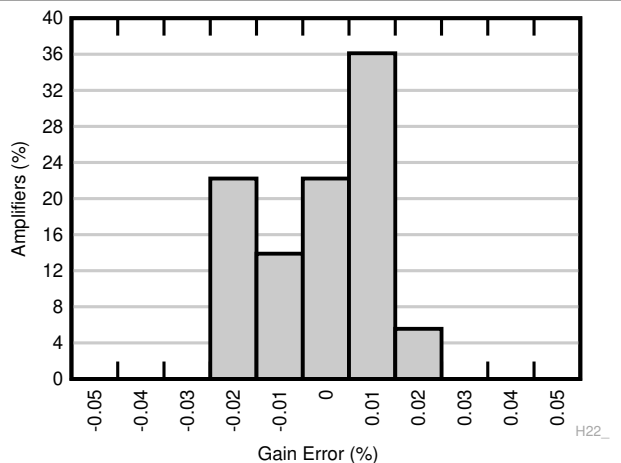
图 6-12. Typical Distribution of Gain Error
