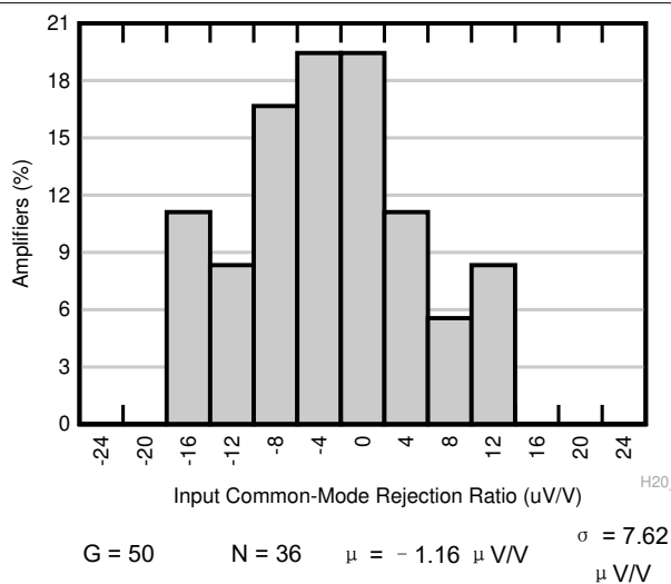
图 6-10. Typical Distribution of CMRR
