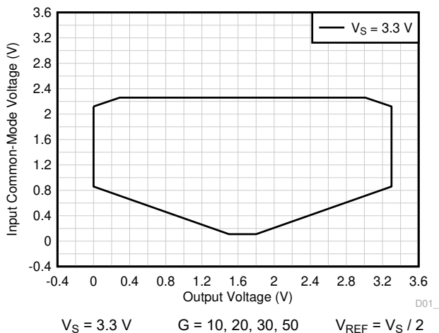
图 6-58. Input Common-Mode Voltage vs Output Voltage (High CMRR Region)
