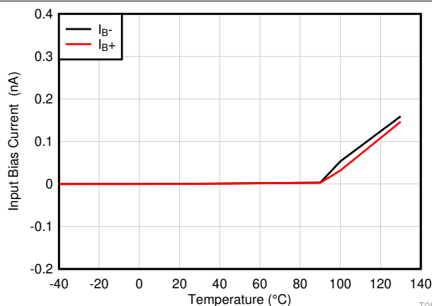
图 6-16. Input Bias Current vs Temperature
