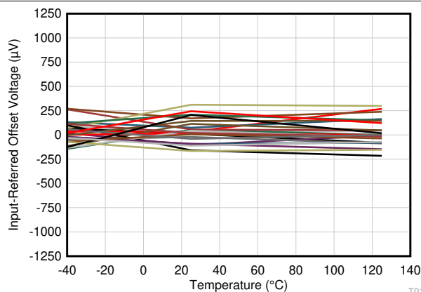
图 6-15. Input Referred Offset Voltage vs Temperature
