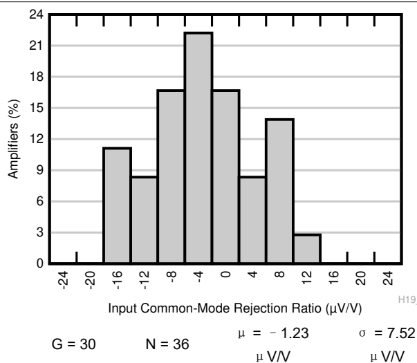
图 6-9. Typical Distribution of CMRR
