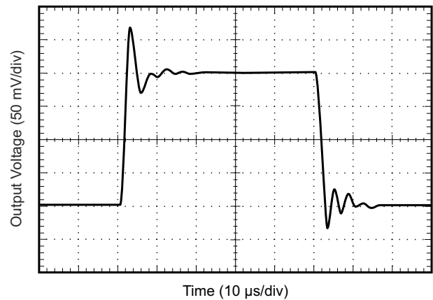
图 6-10. Large Signal Response
