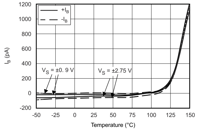
图 6-26. Input Bias Current vs Temperature
