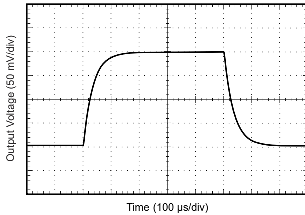
图 6-13. Small-Signal Step Response
