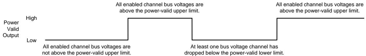
图 19. Power-Valid State Diagram
