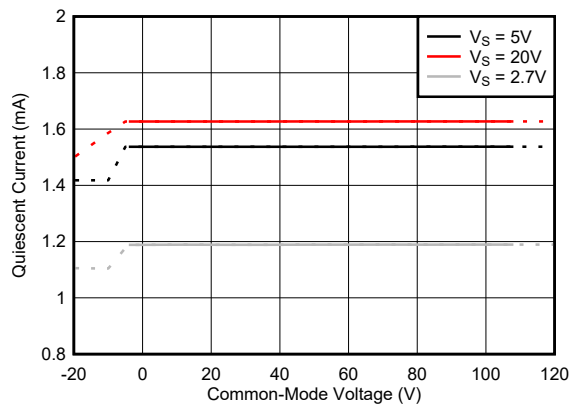
图 6-29. Quiescent Current vs Common-Mode Voltage
