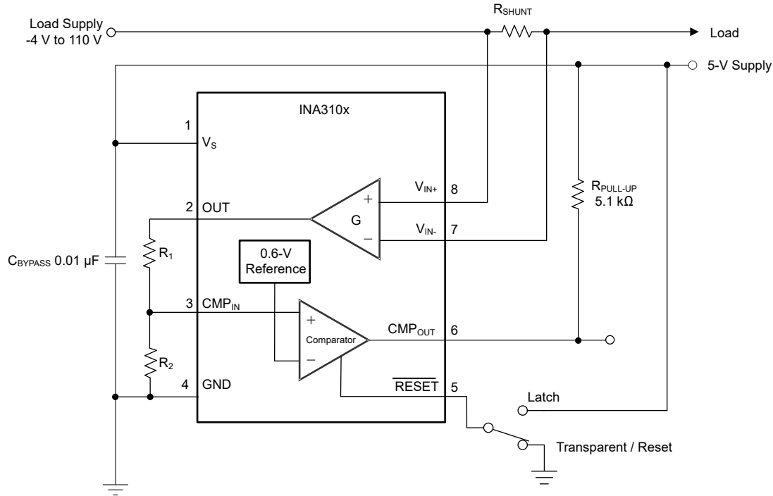
图 7-4. INA310 Basic Connections
