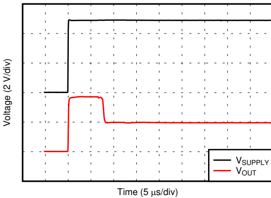
图 6-27. Start-Up Response
