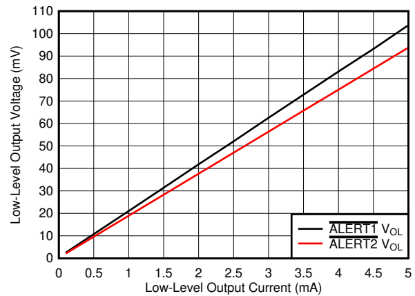
图 6-38. Comparator Alert V_{\text{OL}} vs. I_{\text{OL}}
