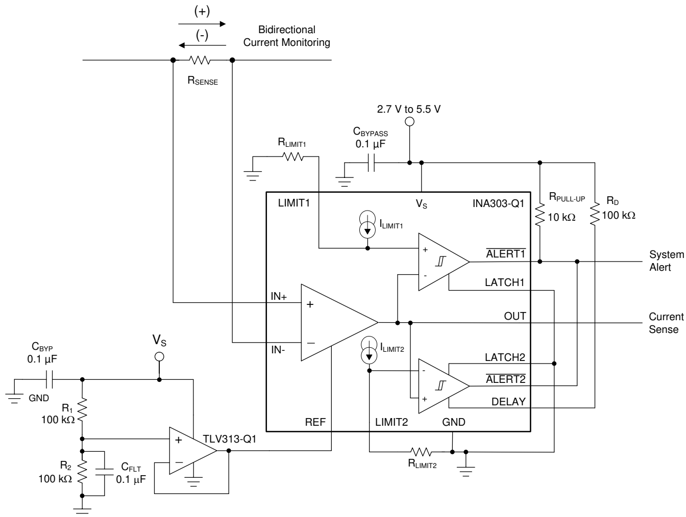
图 8-5. Bidirectional Application
