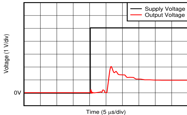
图 6-33. Start-Up Response
