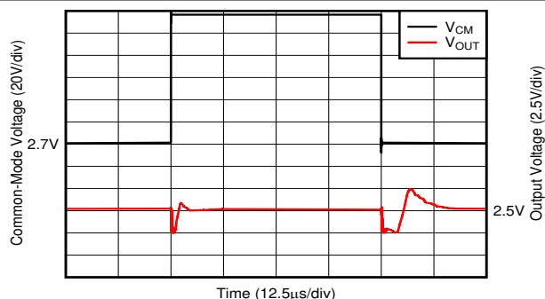
图 6-31. Common-Mode Voltage Fast Transient Pulse, A5 DeviceAs
