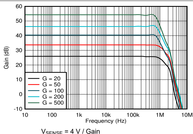
图 6-9. Gain vs Frequency
