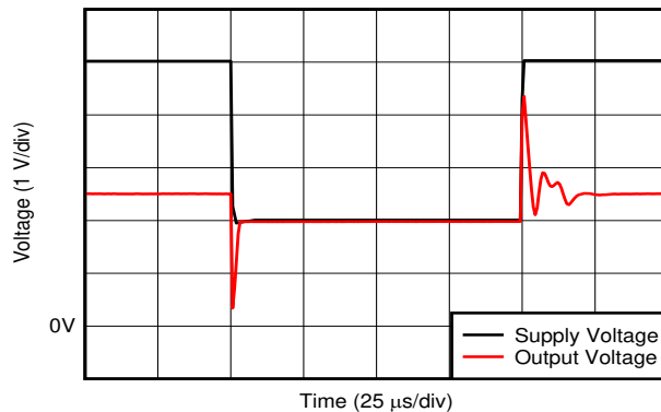
图 6-34. Supply Transient Response, A5 Devices
