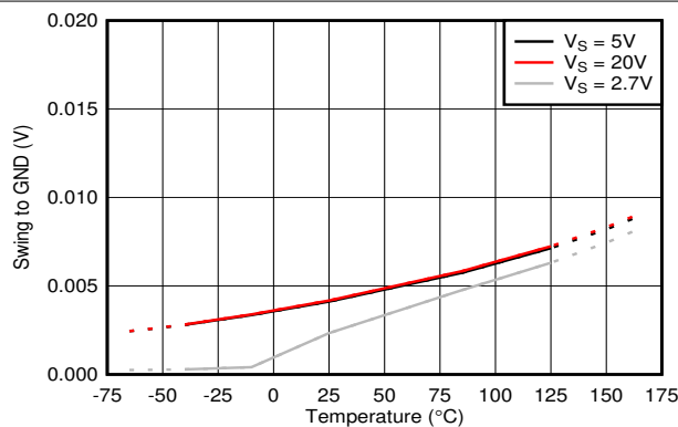
图 6-23. Swing to GND vs Temperature
