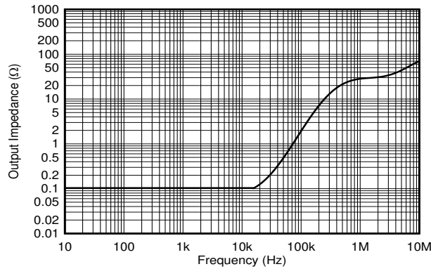
图 6-21. Output Impedance vs Frequency
