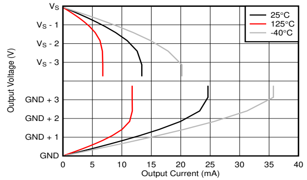
图 6-20. Output Voltage vs Output Current
