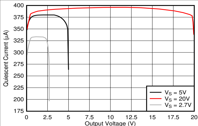
图 6-26. Quiescent Current vs Output Voltage, INA290
