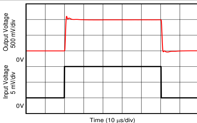
图 6-32. Step Response, A3 Devices
