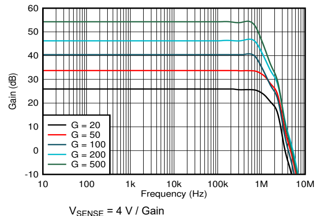
图 6-10. Gain vs. Frequency
