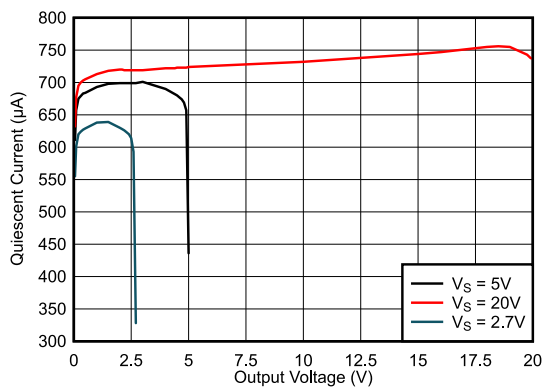
图 6-29. Quiescent Current vs. Output Voltage, INA290
