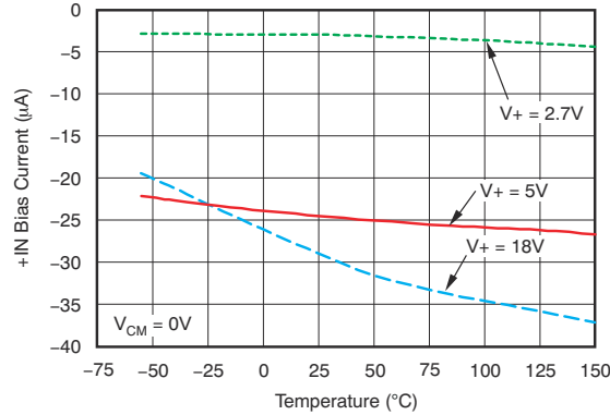
图 6-13. +IN BIAS Current vs Temperature
