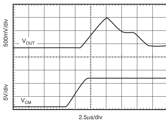
图 6-22. 12-V Common-Mode Step Response
