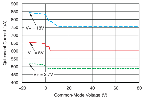
图 6-8. INA283-Q1 Quiescent Current vs Common-Mode Voltage
