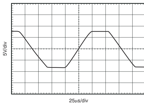
图 6-30. 17-V Step Response
