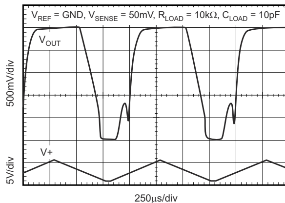
图 6-20. Start-Up Transient Response
