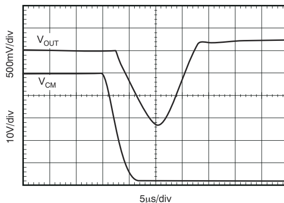
图 6-26. 50-V Common-Mode Step Response
