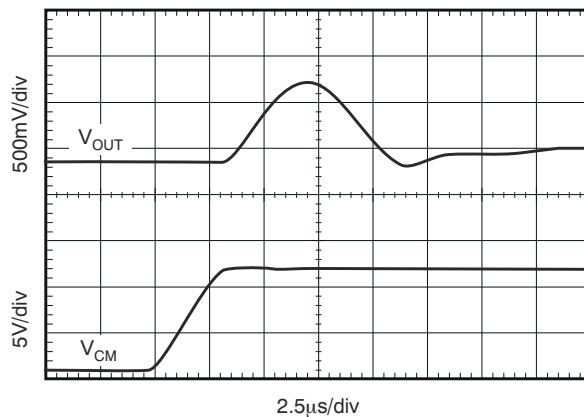
图 6-24. 12-V Common-Mode Step Response
