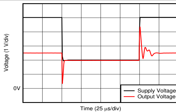
图 6-26. Supply Transient Response, A5 Devices
