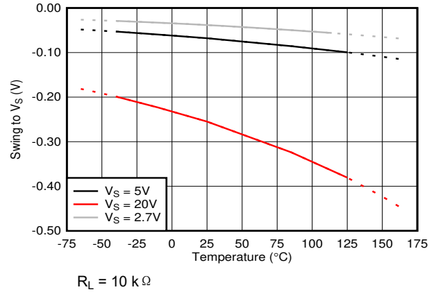
图 6-14. Swing to Supply vs Temperature
