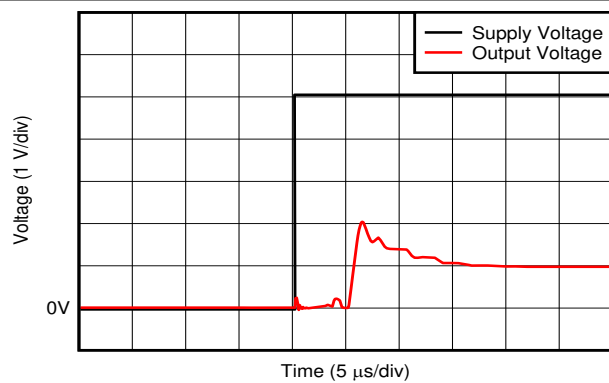
图 6-25. Start-Up Response
