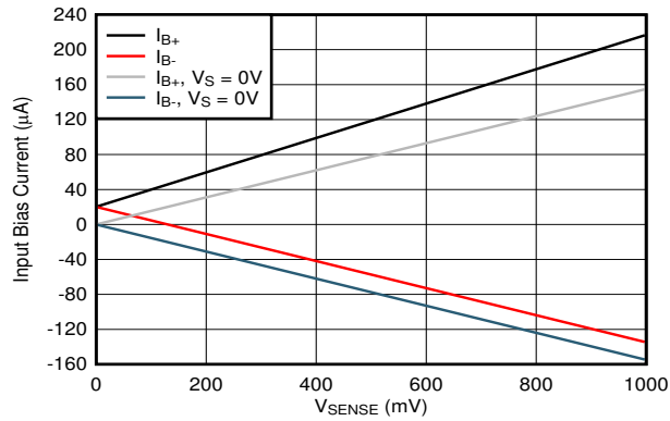
图 6-7. Input Bias Current vs V_{SENSE} , A1 Devices
