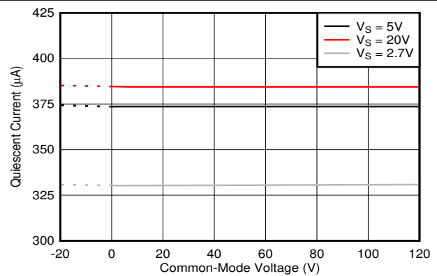
图 6-22. Quiescent Current vs Common-Mode Voltage
