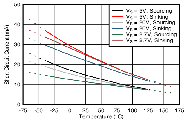
图 6-20. Short-Circuit Current vs Temperature
