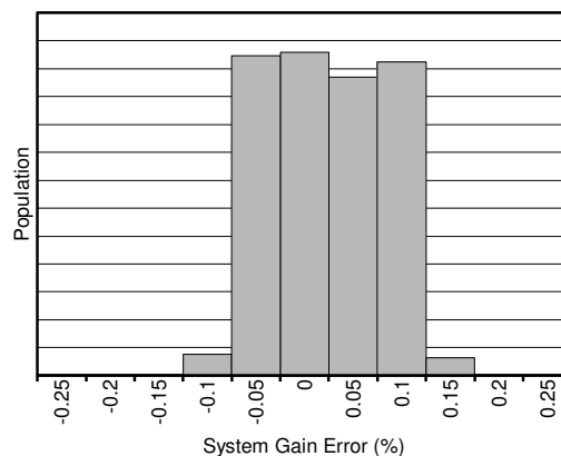
图 6-14. System Gain Error Distribution
