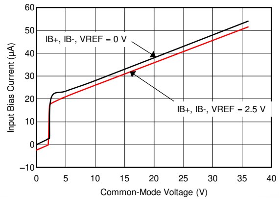
图 6-20. Input Bias Current vs Common-Mode Voltage (VS = 5 V)
