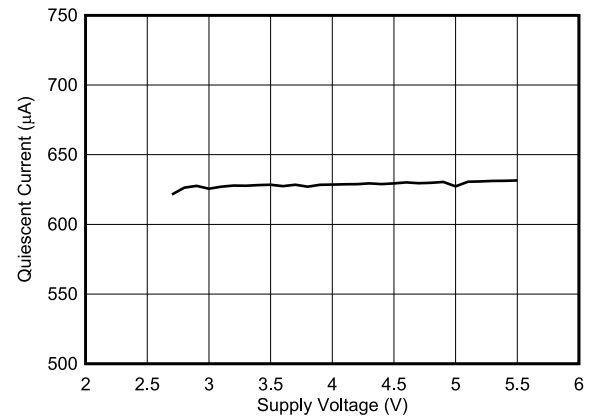
图 6-19. Active I_Q vs. Supply Voltage
