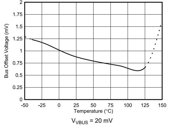
图 6-11. Bus Input Offset Voltage vs. Temperature
