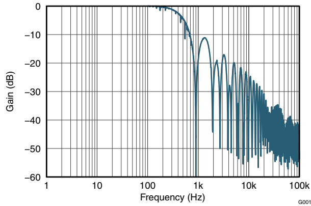
图 5-1. Frequency Response
