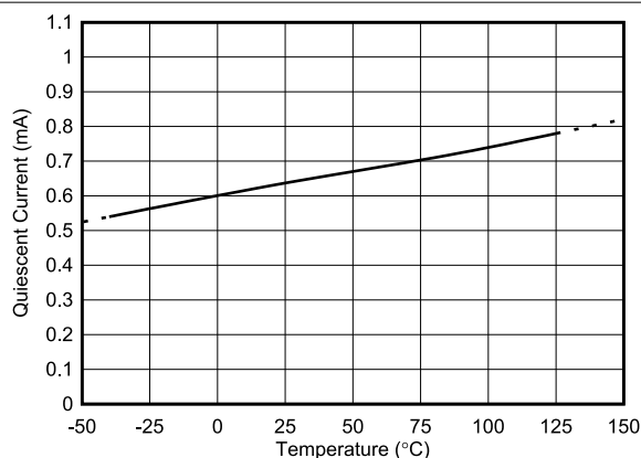
图 6-18. Active I_Q vs. Temperature
