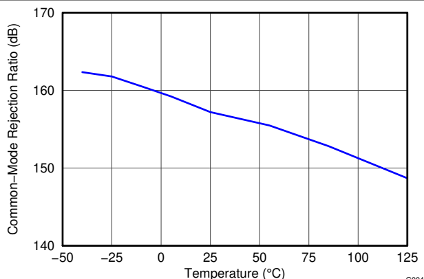
图 5-4. Shunt Input Common-Mode Rejection Ratio vs Temperature
