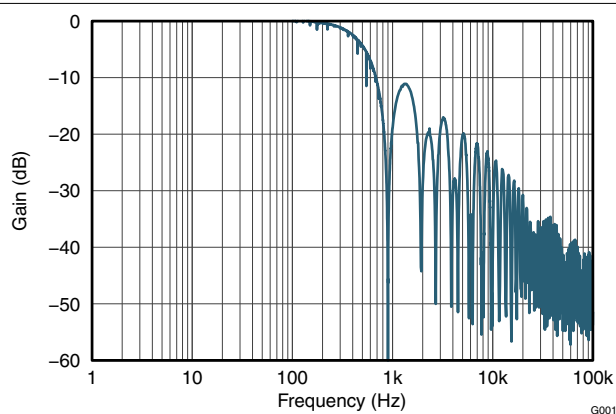
图 5-1. Frequency Response
