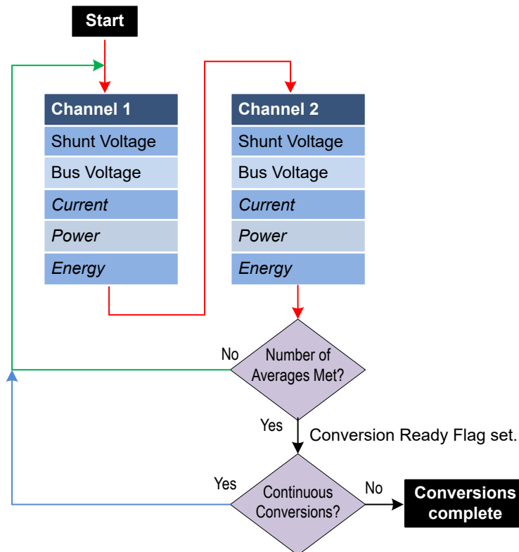
Figure 6-1. Internal Measurement and Calculation Scheme
