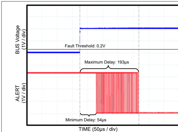
Figure 8-4. Alert Response Time (Sampled Values Significantly Above Threshold)
