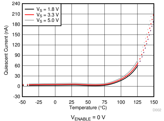
图 6-20. Quiescent Current vs. Temperature (INA191 Disabled)
