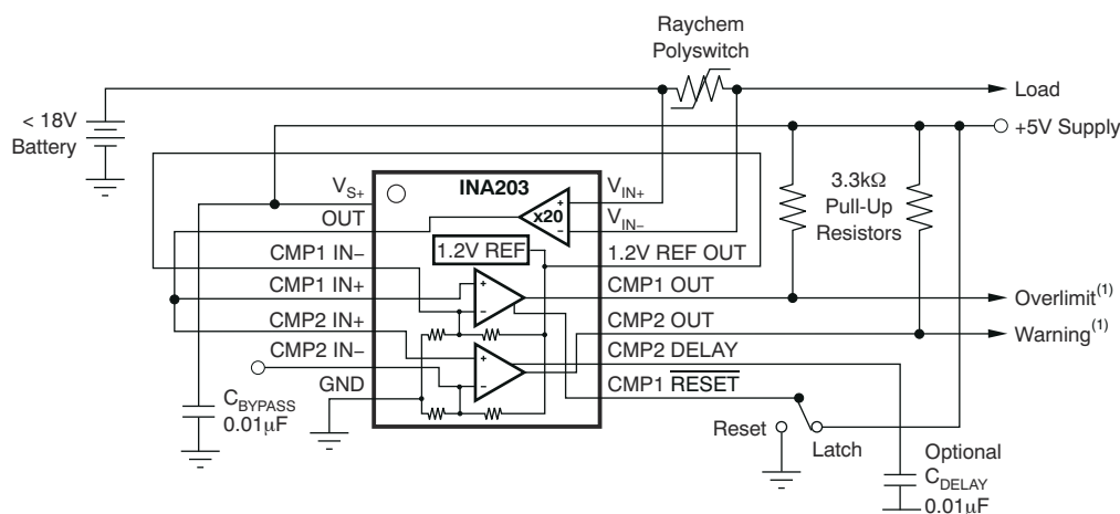
图 8-1. Polyswitch Warning and Fault Detection Circuit
