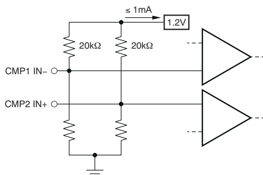
图 7-6. Limit Current Into Reference \leq 1\text{ mA}
