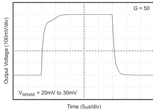
图 6-15. Step Response
