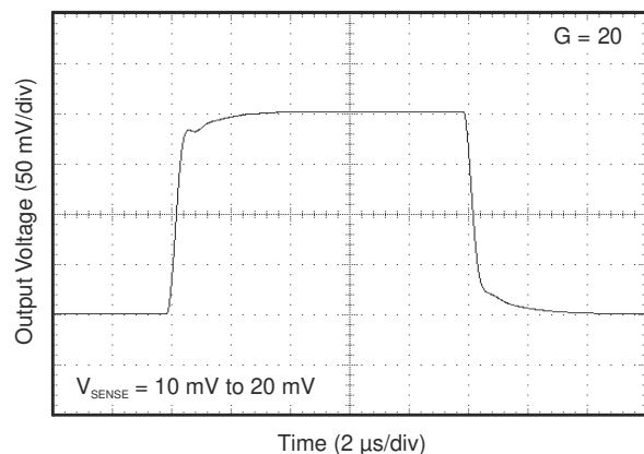
图 6-13. Step Response
