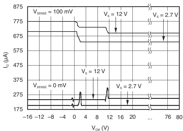
图 6-11. Quiescent Current vs Common Mode Voltage
