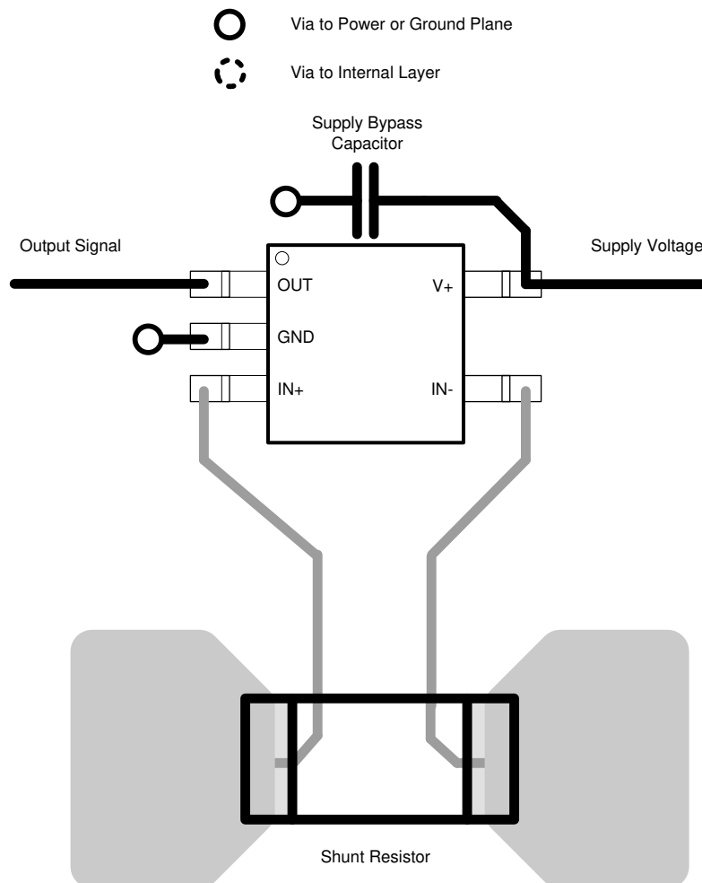
图 10-1. Recommended Layout
