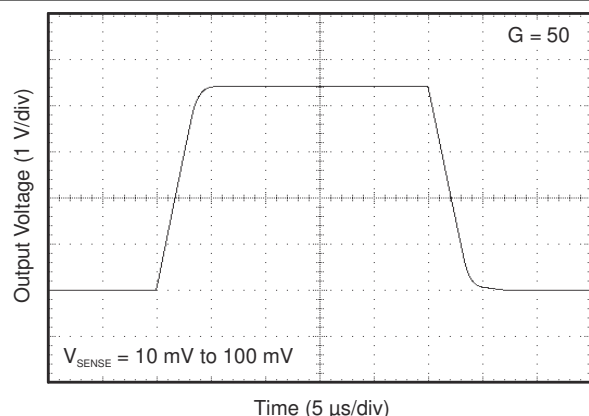
图 6-17. Step Response
