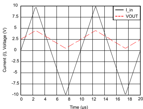
图 8-2. Output Voltage vs Shunt Input Current
