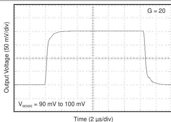
图 6-15. Step Response
