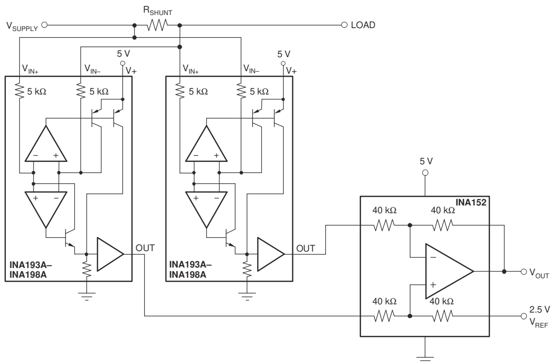
图 7-3. Bidirectional Current Monitoring
