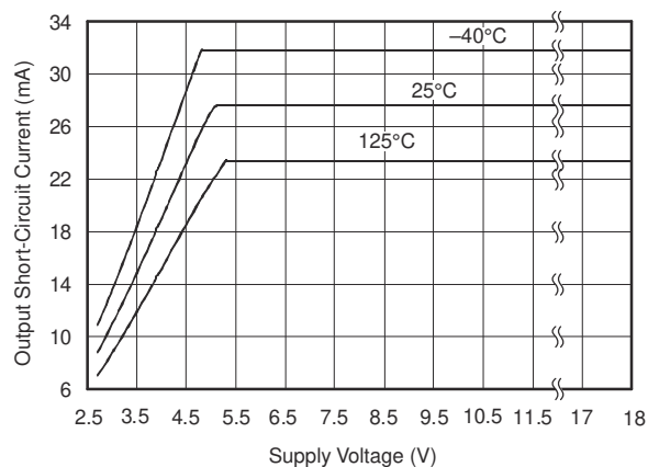
图 6-12. Output Short Circuit Current vs Supply Voltage
