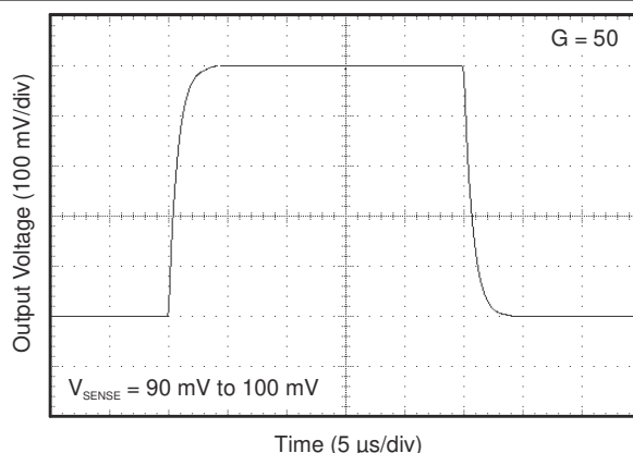
图 6-18. Step Response
