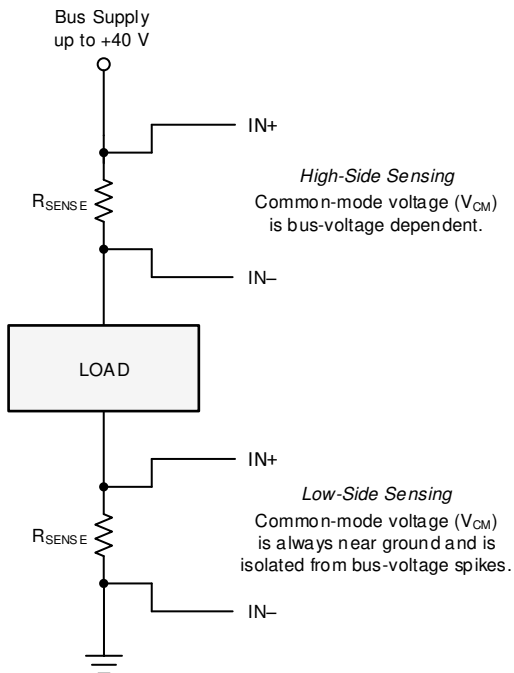
图 7-1. High-Side and Low-Side Sensing Connections
