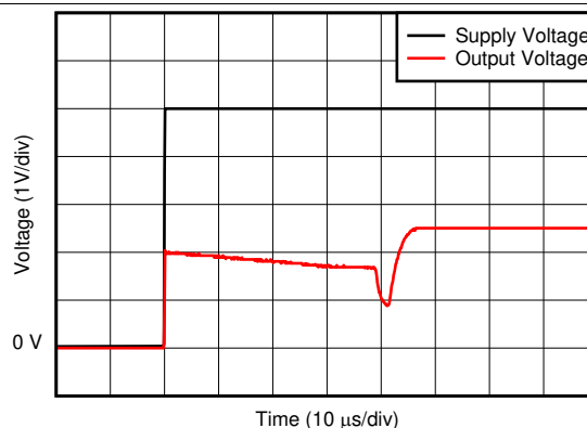
图 26. Start-Up Response
