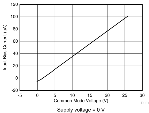
图 5-21. Input Bias Current vs Common-Mode Voltage (Both Inputs, Shutdown) Supply voltage = 0 V
