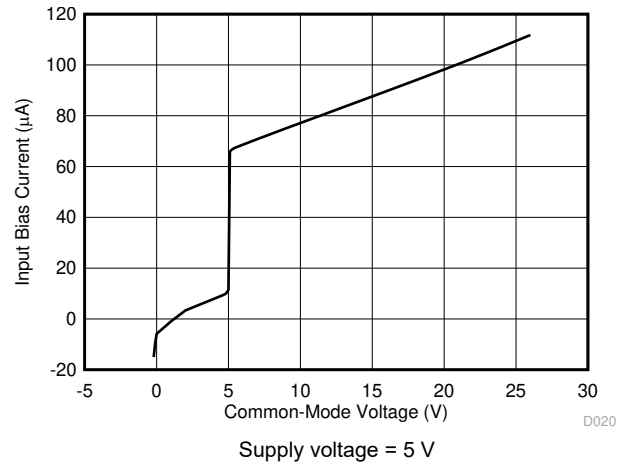
图 5-20. Input Bias Current vs Common-Mode Voltage Supply voltage = 5 V
