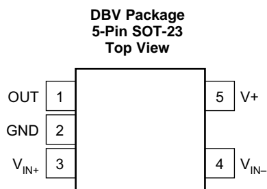
Pin Functions
