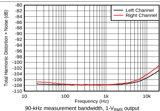
图 58. THD+N vs Frequency for a 32- \Omega Load
