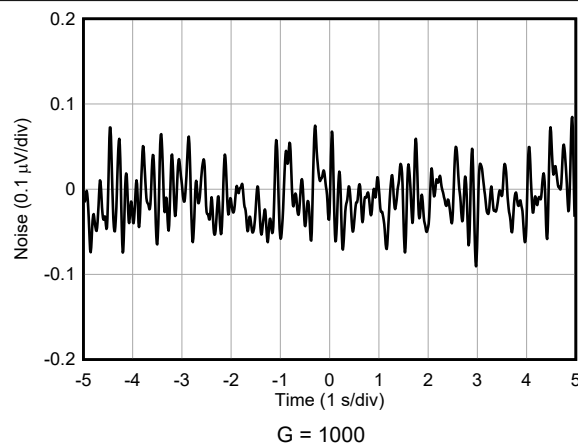
图 7-20. Input-Referred Noise, 0.1 Hz to 10 Hz
