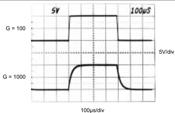
图 7-22. Small-Signal Response
