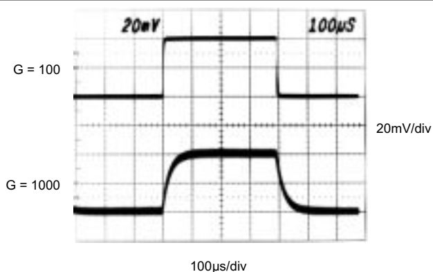
图 7-22. Small-Signal Response
