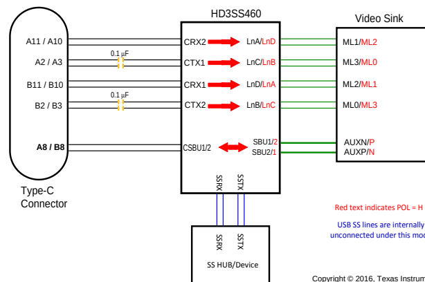
RECEPTACLE PIN NUMBER 460 PIN MAPPING TO TYPE C CONNECTOR 460 PIN MAPPING TO DP SOURCE (GPU) POL = L POL = H A11/10 CRX2 LnA(ML1) LnD(ML2) A2/3 CTX1 LnC(ML3) LnB(ML0) B11/10 CRX1 LnD(ML2) LnA(ML1) B2/3 CTX2 LnB(ML0) LnC(ML3) A8 CSBU1 SBU1(AUXN) SBU2(AUXP) B8 CSBU2 SBU2(AUXP) SBU1(AUXN)
