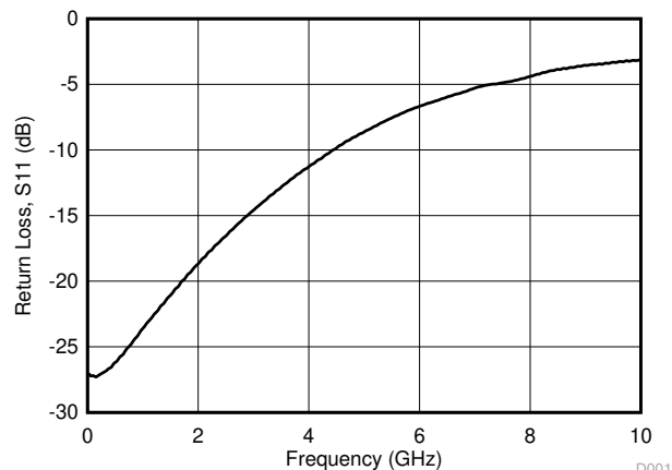
图 5-1. Return Loss vs Frequency
