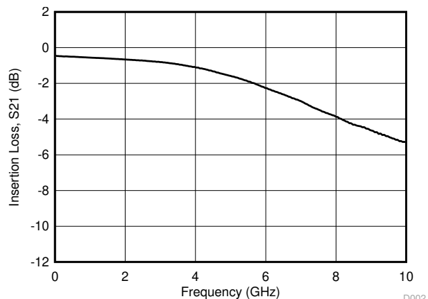
图 5-2. Insertion Loss vs Frequency
