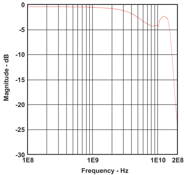
图 9-5. Insertion Loss and -3dB Bandwidth
