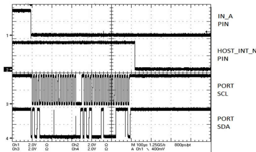
图 8-6. Interrupt-Driven Pre-Fetch
