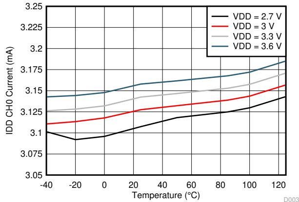
图 5-2. Active Mode I_{DD} vs Temperature
