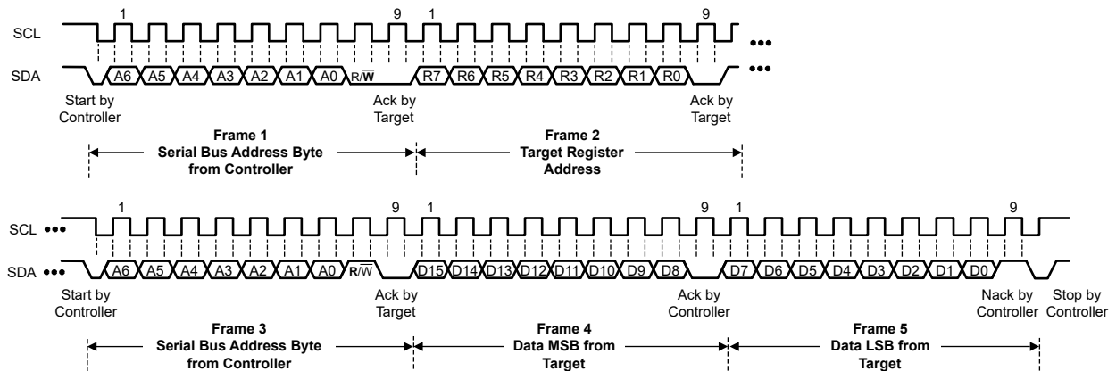
图 6-7. I 2 C Read Register Sequence
