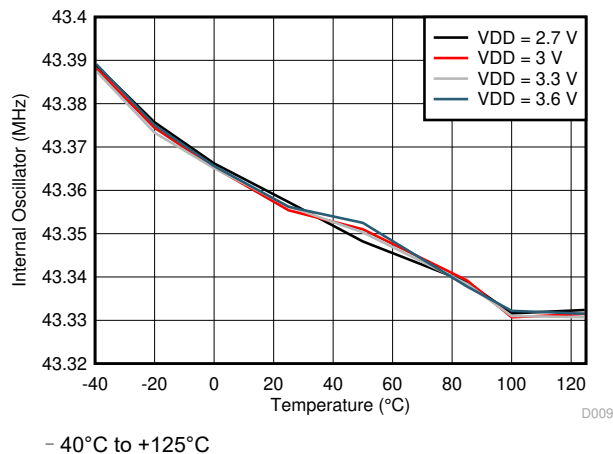
图 5-8. Internal Oscillator Frequency vs Temperature
