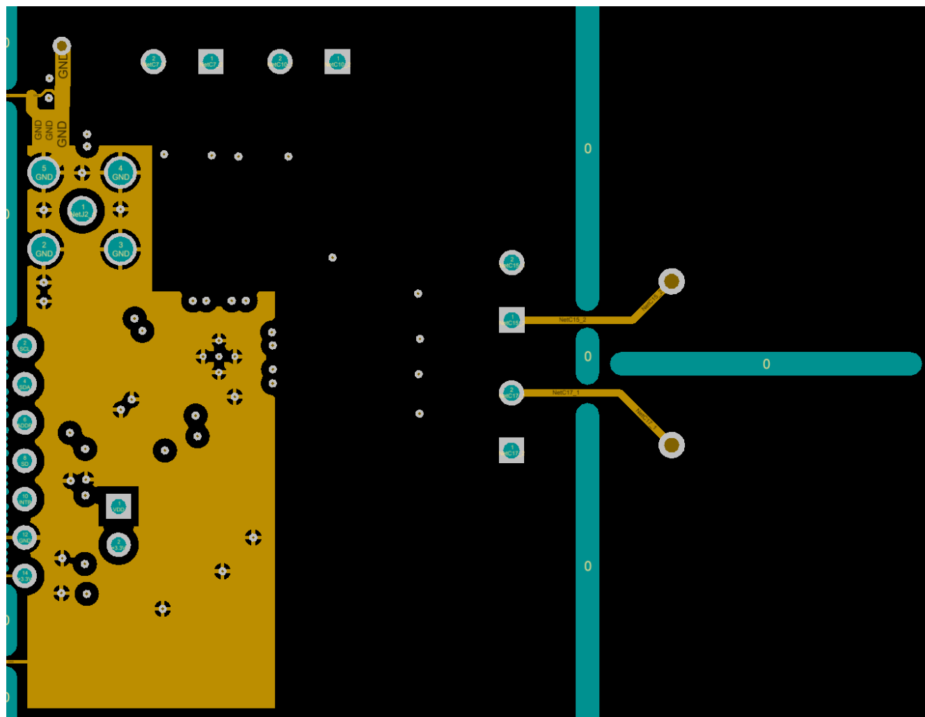
图 7-10. Example PCB Layout: Mid-Layer 1 (GND)
