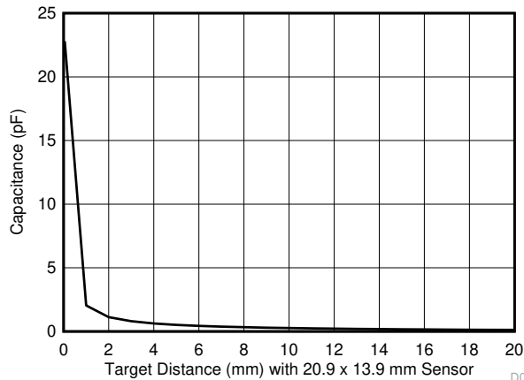
图 7-4. FDC2212 / FDC2214: Capacitance vs Target Distance (0mm to 20mm)
