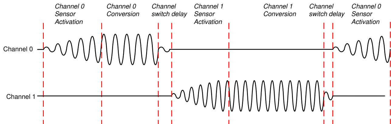
图 6-4. Multi-Channel Mode Sequencing
