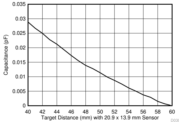
图 7-6. FDC2212 / FDC2214: Capacitance vs Target Distance (40mm to 60mm)
