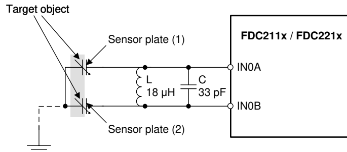
图 7-2. Differential Sensor Configuration
