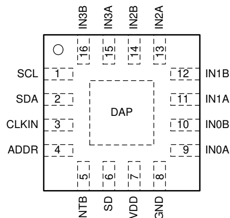
图 4-2. FDC2114/FDC2214 RGH Package 16-Pin WQFN Top View
