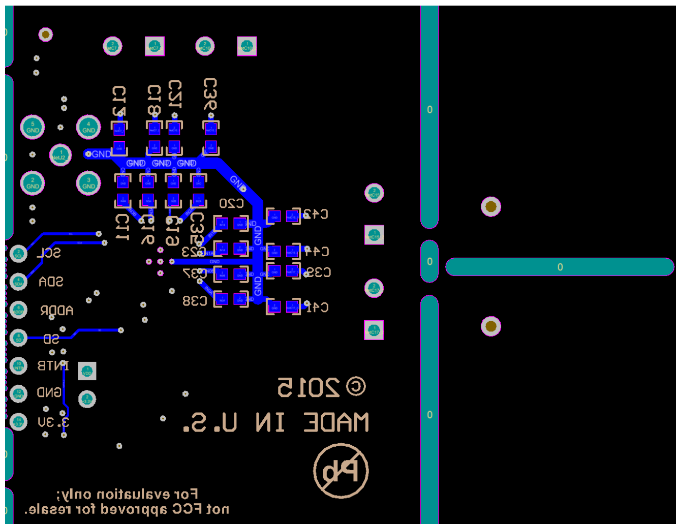
图 7-12. Example PCB Layout: Bottom Layer (Signal)
