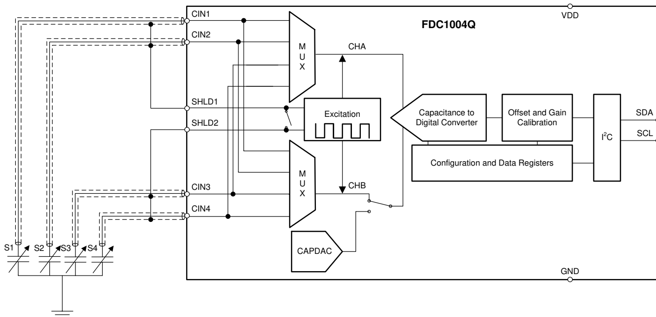
图 6-3. Differential Configuration
