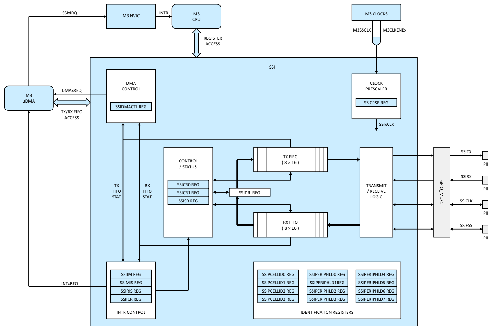
Figure 5-31. SSI
