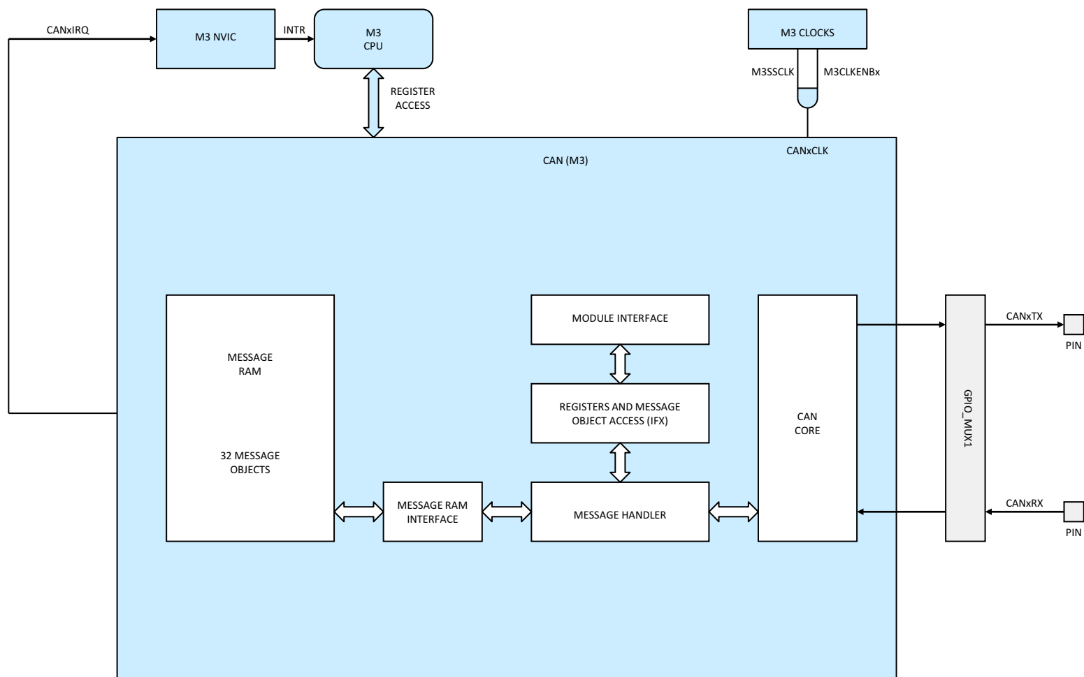
Figure 5-34. CAN (Cortex-M3)
