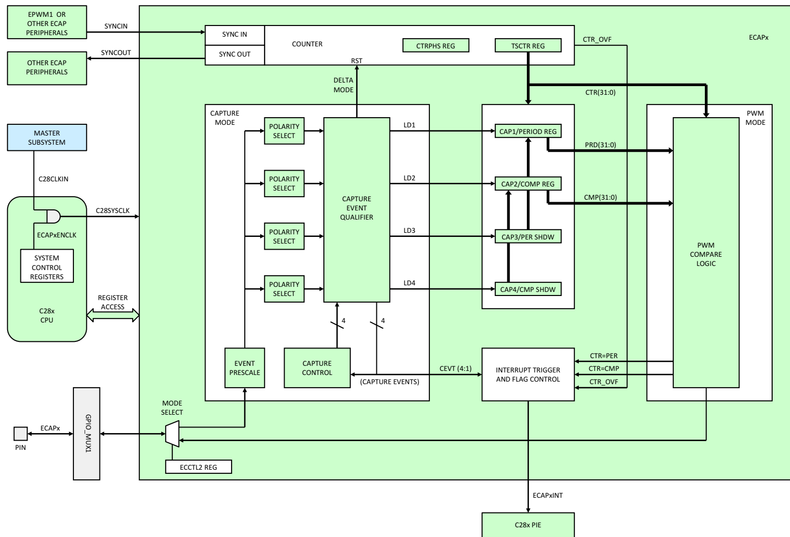
Figure 5-47. eCAP
