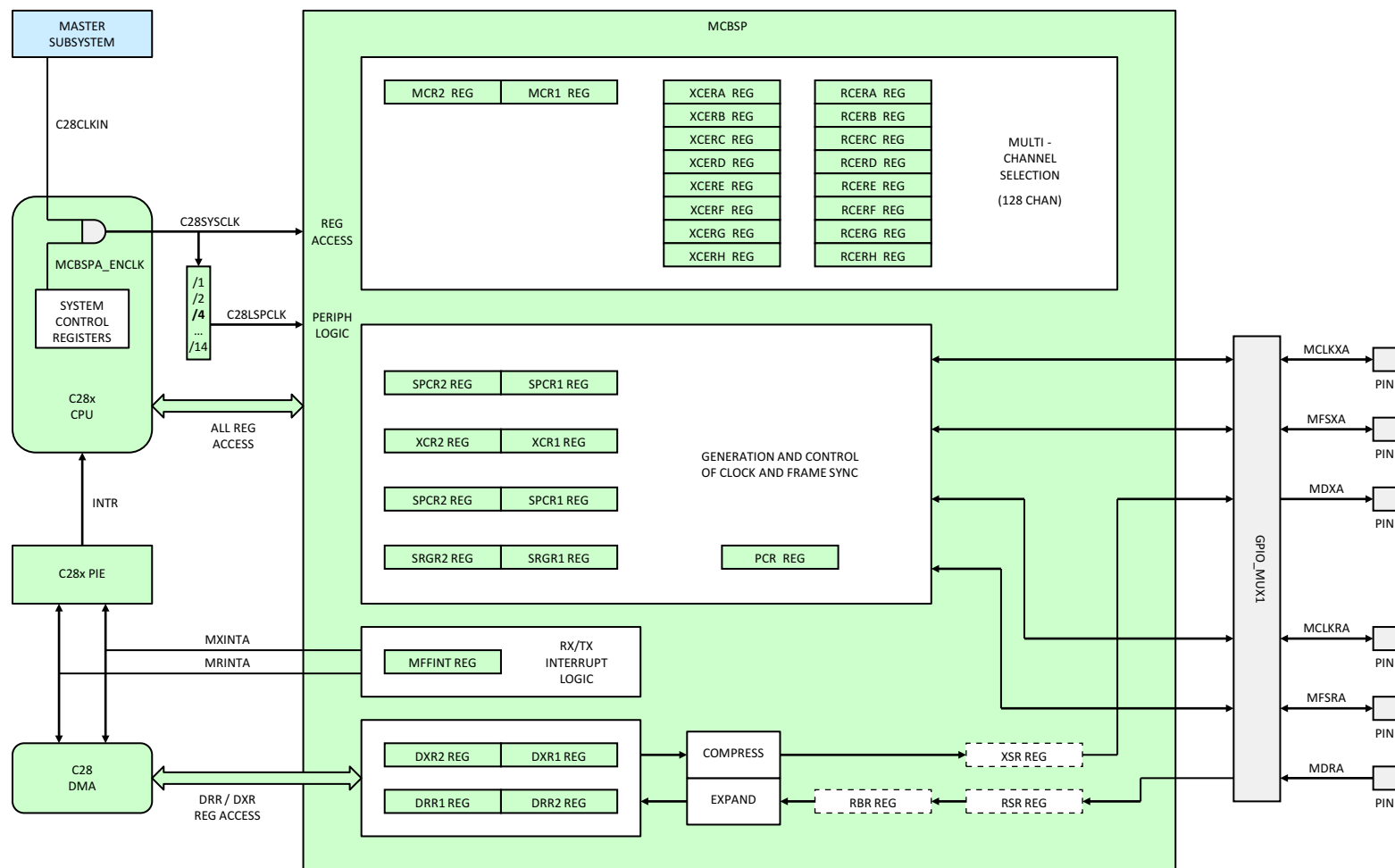
Figure 5-56. McBSP (C28x)
