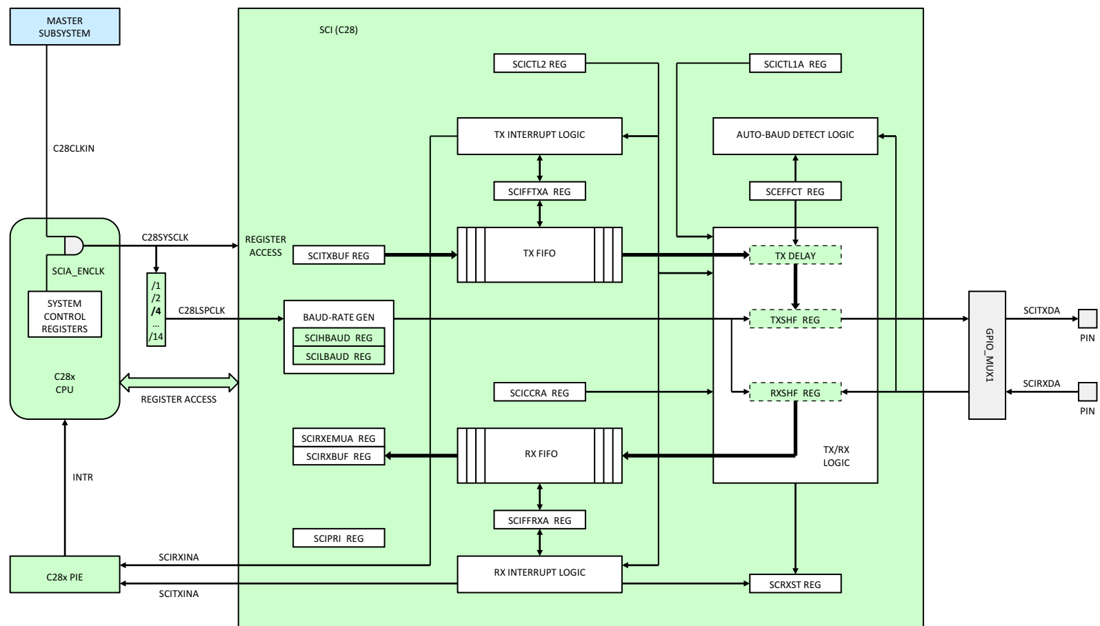
Figure 5-50. SCI (C28x)
