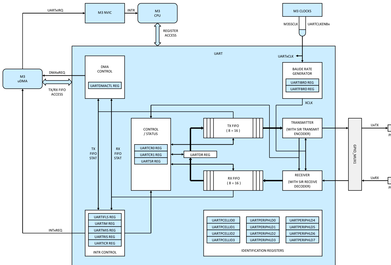
Figure 5-32. UART
