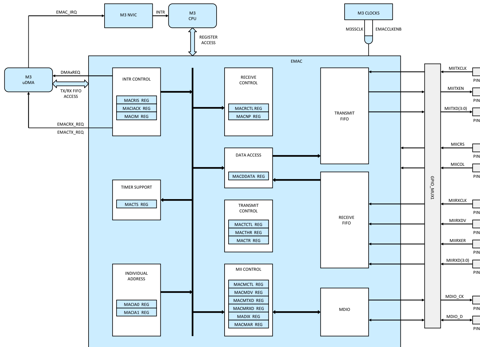
Figure 5-36. EMAC
