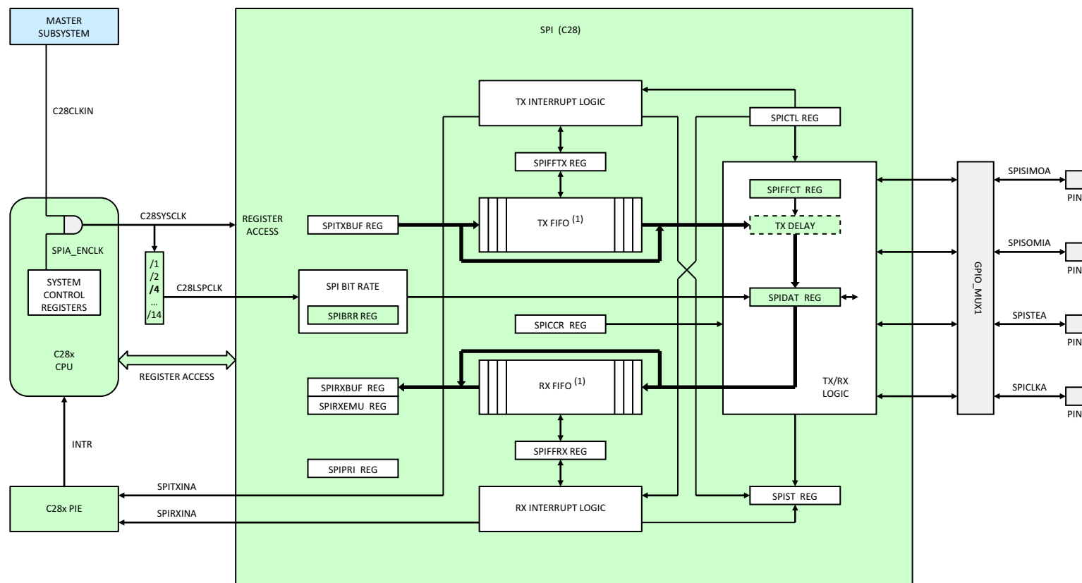
Figure 5-51. SPI (C28x)
