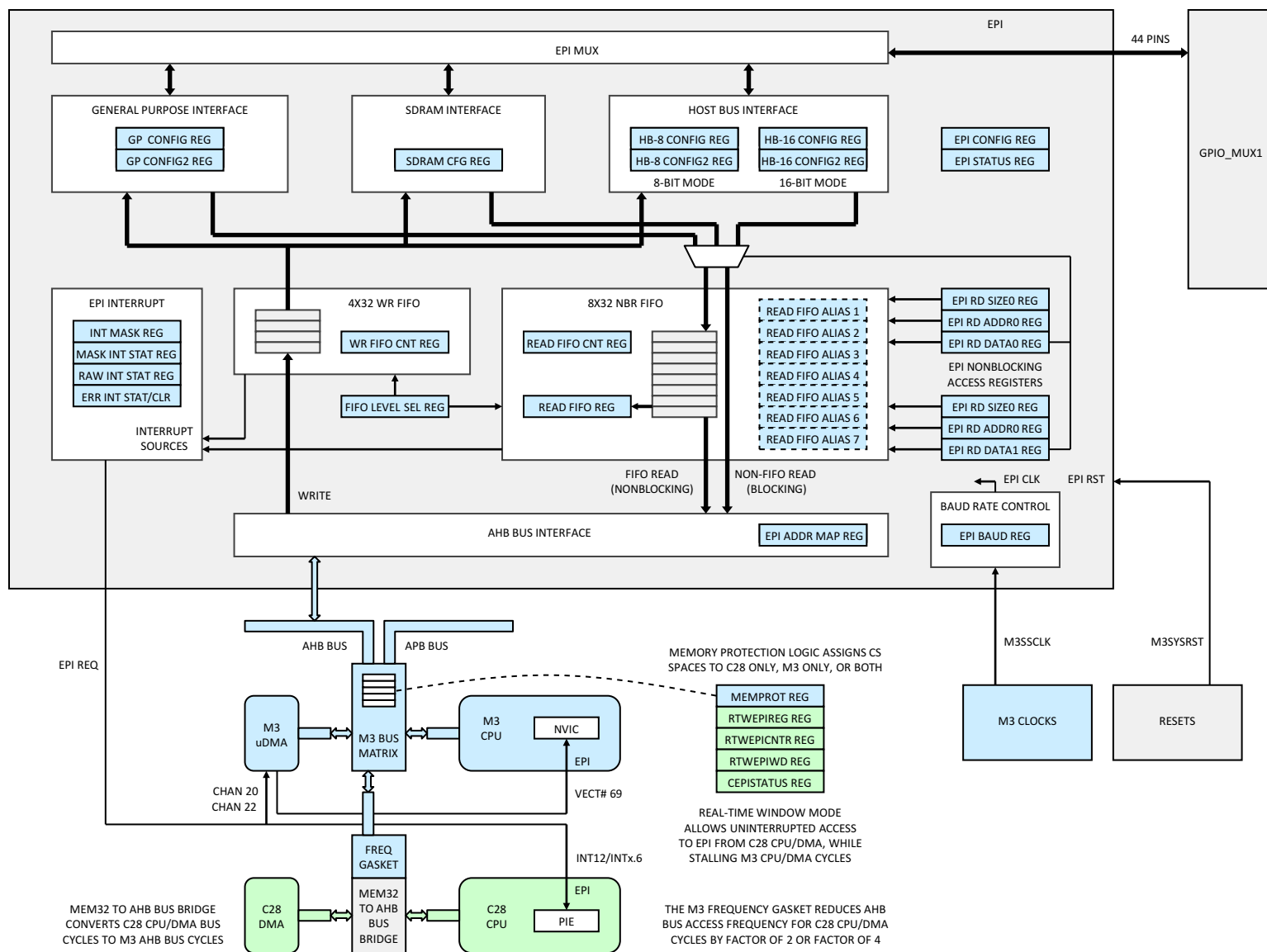
Figure 5-17. EPI
