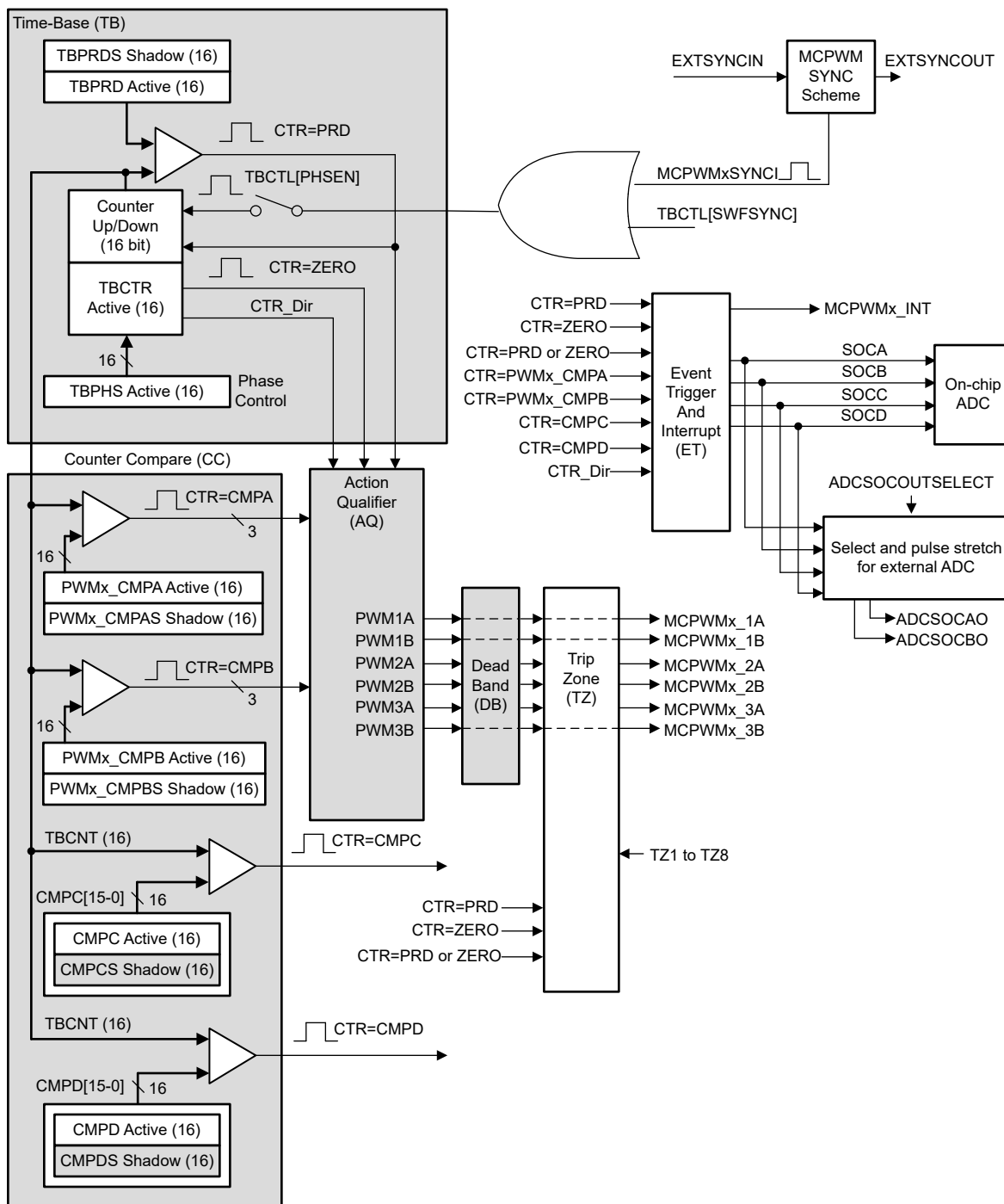
Figure 6-47. MCPWM Submodules and Critical Internal Signal Interconnects
