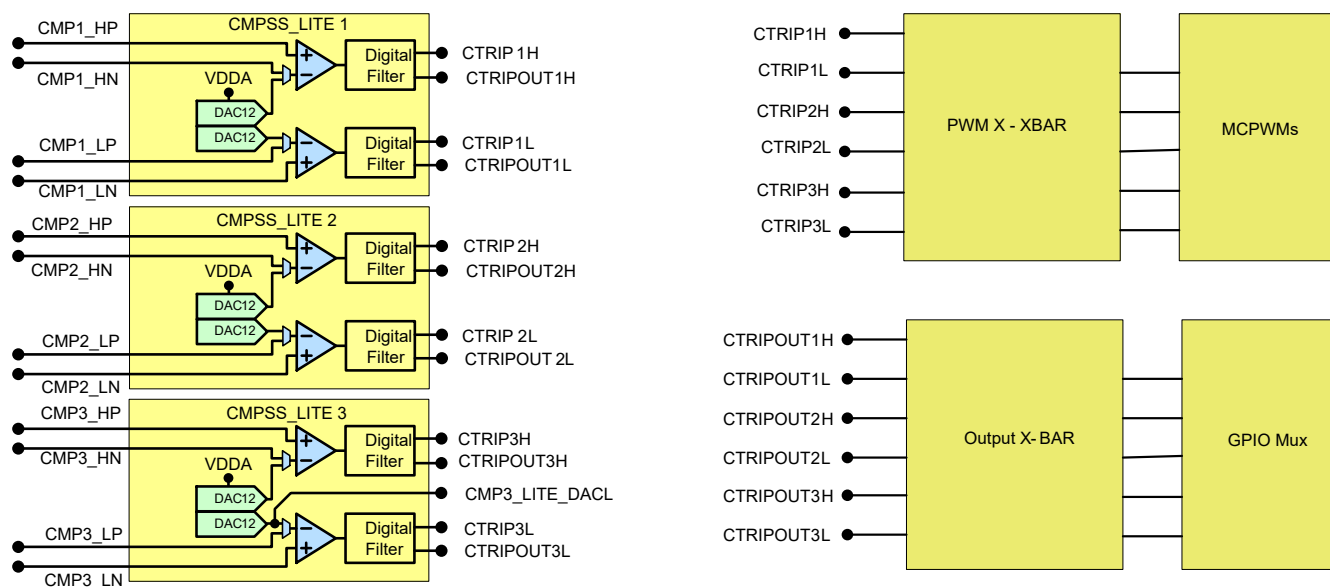
Figure 6-38. CMPSS Connectivity
