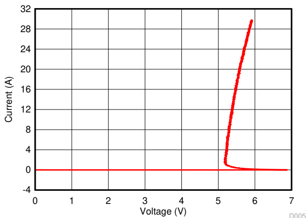
图 5-5. TLP I-V Curve, IO to GND, t_p = 100ns
