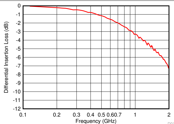
图 5-12. Differential Insertion Loss
