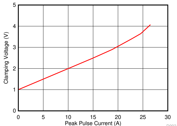
图 5-2. Clamping Voltage vs. Peak Pulse Current ( t_p = 8/20\mu s ), GND to Any IO Pin
