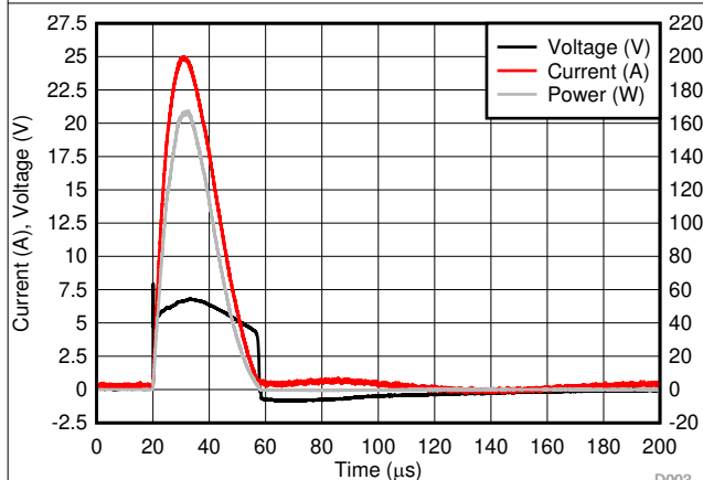
图 5-3. Surge Current, Clamping Voltage and Power Curve ( t_p = 8/20\mu s ), Any IO Pin to GND
