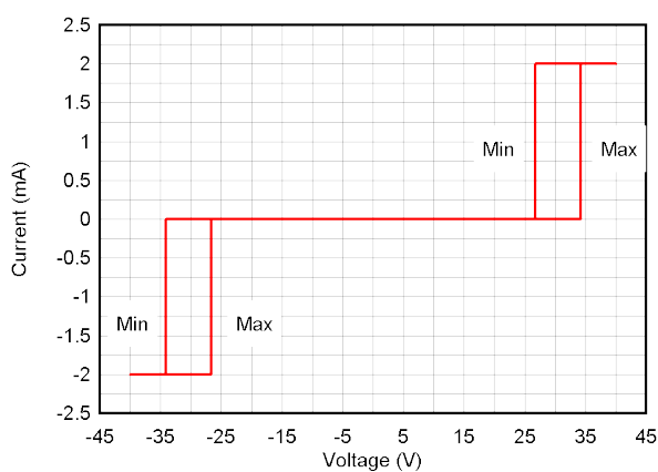
图 6-12. DC Voltage Sweep I-V Curve
