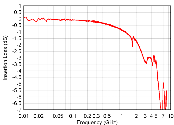
图 6-17. Insertion Loss
