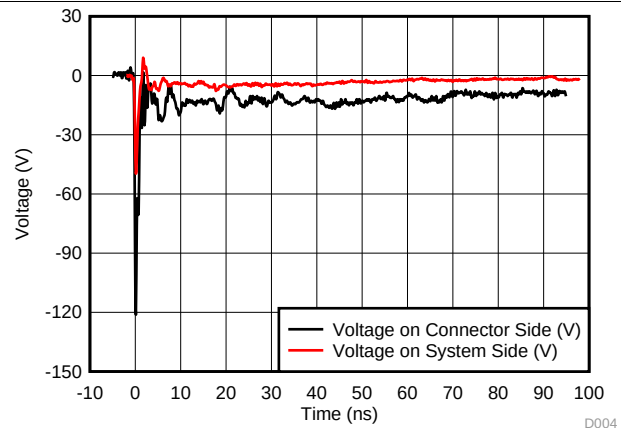
图 4. Clamping voltage waveform for -8kV IEC 61000-4-2 stress. See 图 11 for details.
