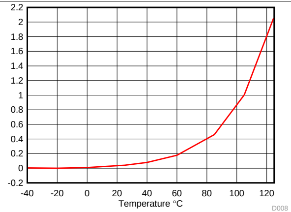
图 8. Leakage Current vs Temperature, IO Pin to GND, at 2.5 V Bias
