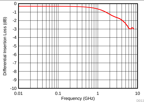
图 9. Differential Insertion Loss
