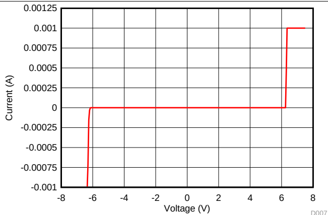
图 7. DC Voltage Sweep I-V Curve, IO Pin to GND
